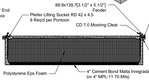
SECTION A-A SCALE 3/8" = 1'
