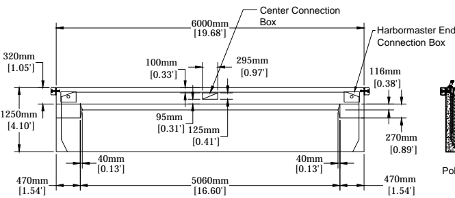
END ELEVATION VIEW
