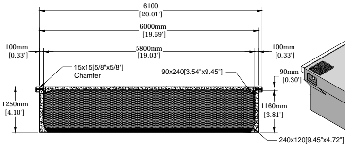
HARBORMASTERS H6200-H SECTION A-A
