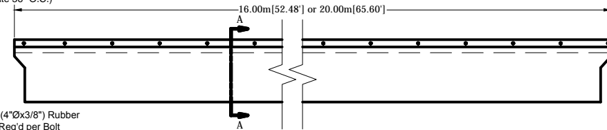
SIDE ELEVATION VIEW
