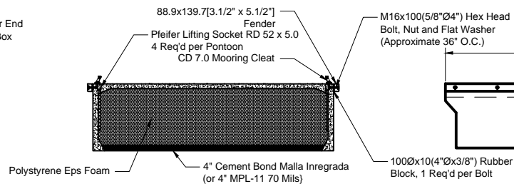
SECTION A-A SCALE 3/8" = 1'
