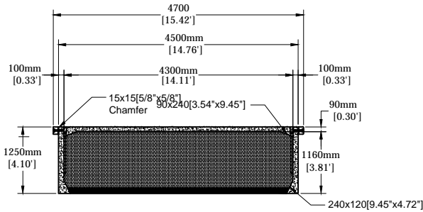
HARBORMASTERS H4800-H SECTION A-A
