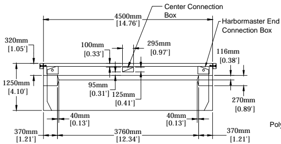
END ELEVATION VIEW
