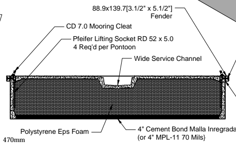
SECTION A-A SCALE 3/8"=1'
