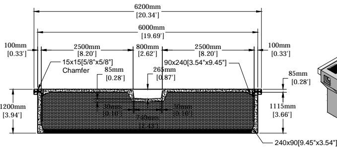
COMMODORE C6200CC SECTION A-A
