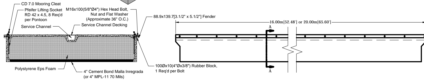
SECTION A-A SCALE 3/8" = 1'
