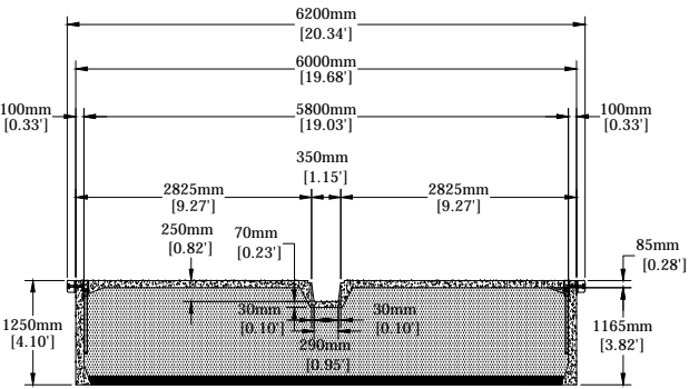
COMMODORE C6200Cc-H SECTION A-A
