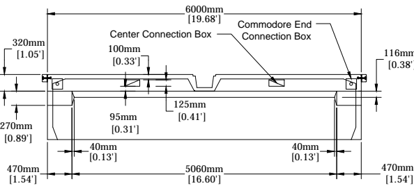
END ELEVATION VIEW
