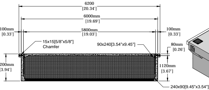
COMMODORE C6200 SECTION A-A
