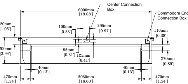
END ELEVATION VIEW
