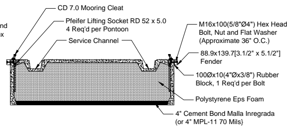
SECTION A-A SCALE 3/8" = 1'
