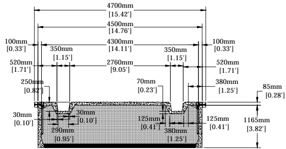
COMMODORE C4800c SECTION A-A
