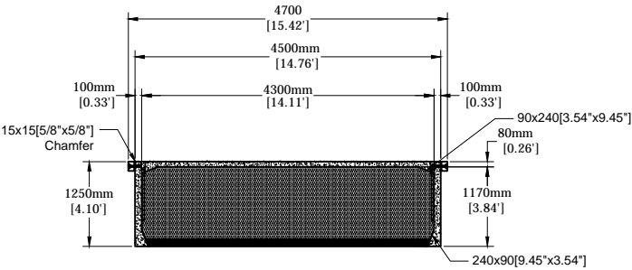
COMMODORE C4800H SECTION A-A
