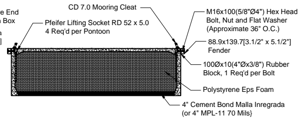
SECTION A-A SCALE 3/8" = 1'
