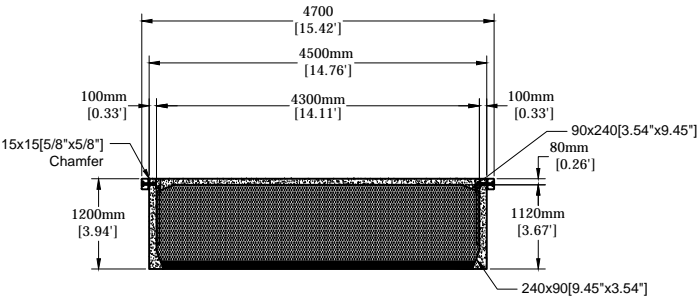
COMMODORE C4800 SECTION A-A
