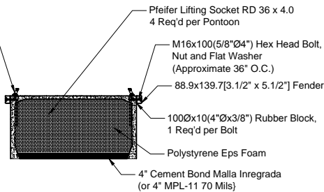
SECTION A-A SCALE 3/8" = 1'
