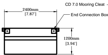
ADMIRAL A2600H SECTION A-A
