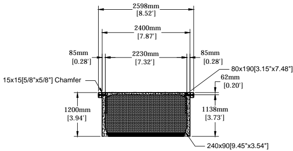
ADMIRAL A2600H SECTION A-A
