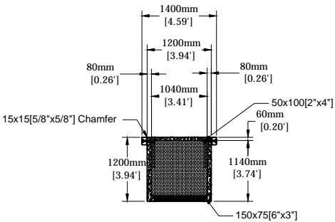
ADMIRAL A1300 SECTION A-A
