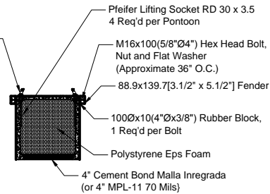
SECTION A-A SCALE 3/8" = 1'
